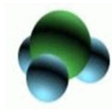
amoniak - NH 3
